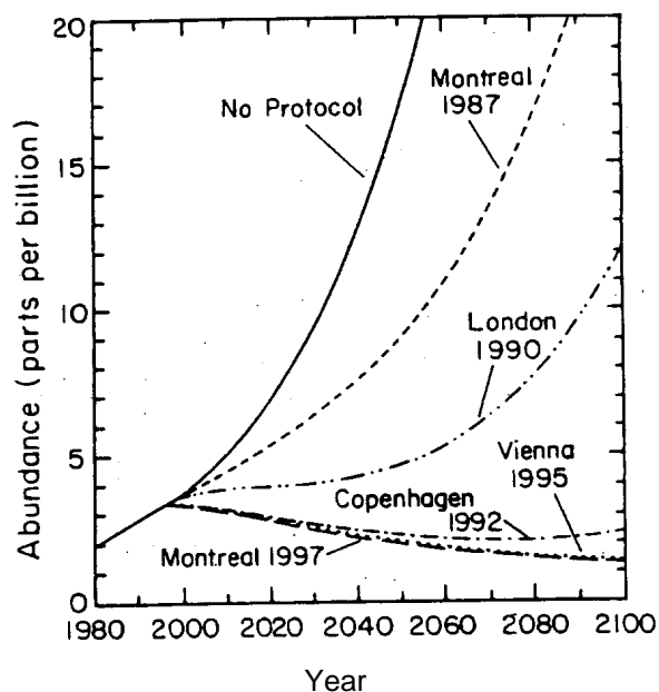
Figure 1. Effect of the international agreements on ozone-depleting stratospheric chlorine/bromine.
