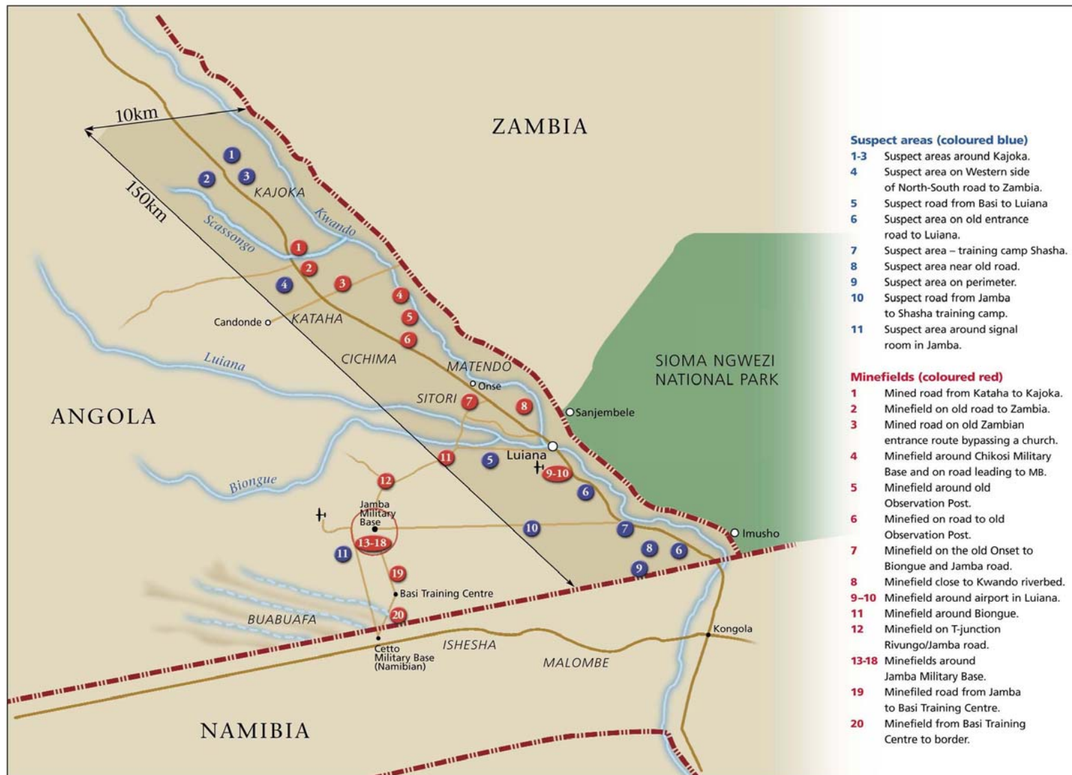
Map showing the distribution of confirmed and suspected minefields in Luiana and the 10 km x 150 km strip to be cleared.
